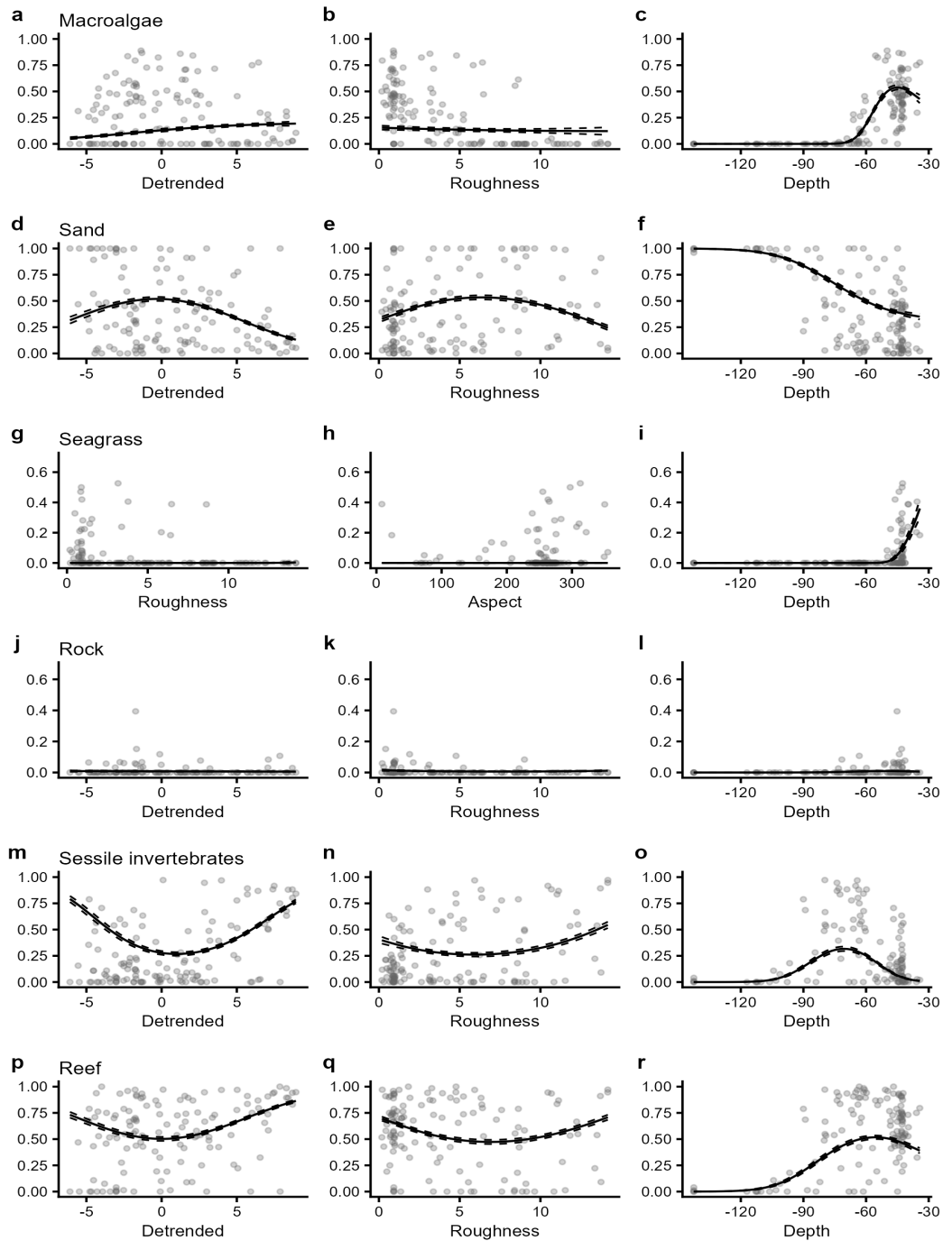
Figure C 1.2.3: Plots of the most parsimonious model found to predict the probability of occurrence of key habitat types in 2024. Individual panes display the predicted relationships between model covariates and the probability of occurrence of each habitat class. Solid lines represent predicted Generalized Additive Model (GAM) fits with other variables held constant at their mean value and survey year held at 2024. Dashed lines represent upper and lower standard error bounds around the prediction, and points represent the observed data for that year.
