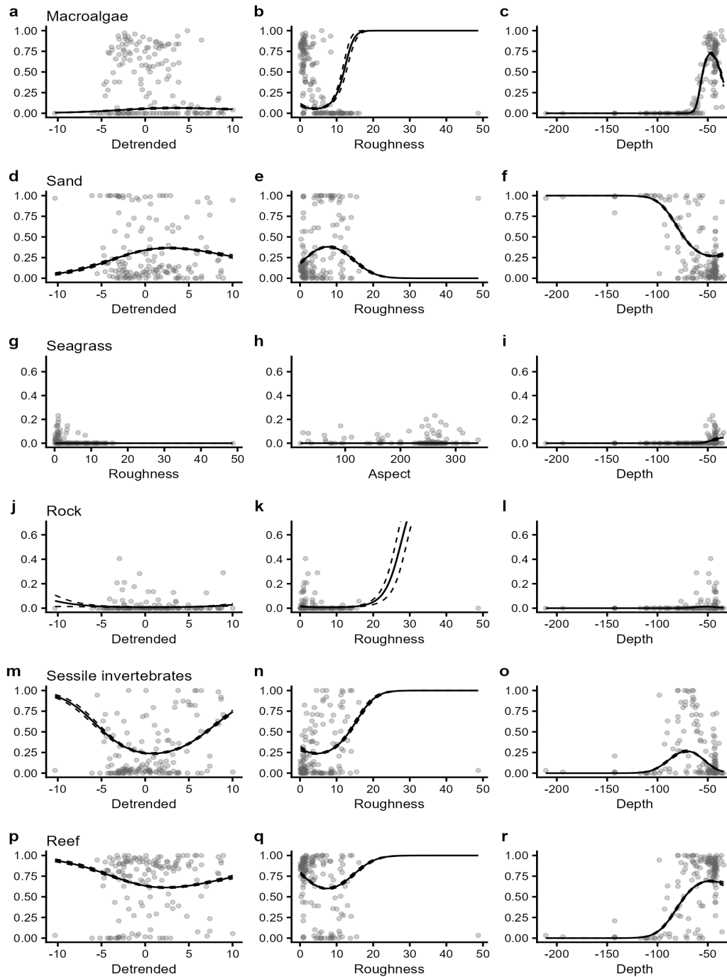
Figure C 1.2.4: Plots of the most parsimonious model found to predict the probability of occurrence of key habitat types in 2025. Individual panes display the predicted relationships between model covariates and the probability of occurrence of each habitat class. Solid lines represent predicted Generalized Additive Model (GAM) fits with other variables held constant at their mean value and survey year held at 2025. Dashed lines represent upper and lower standard error bounds around the prediction, and points represent the observed data for that year.
