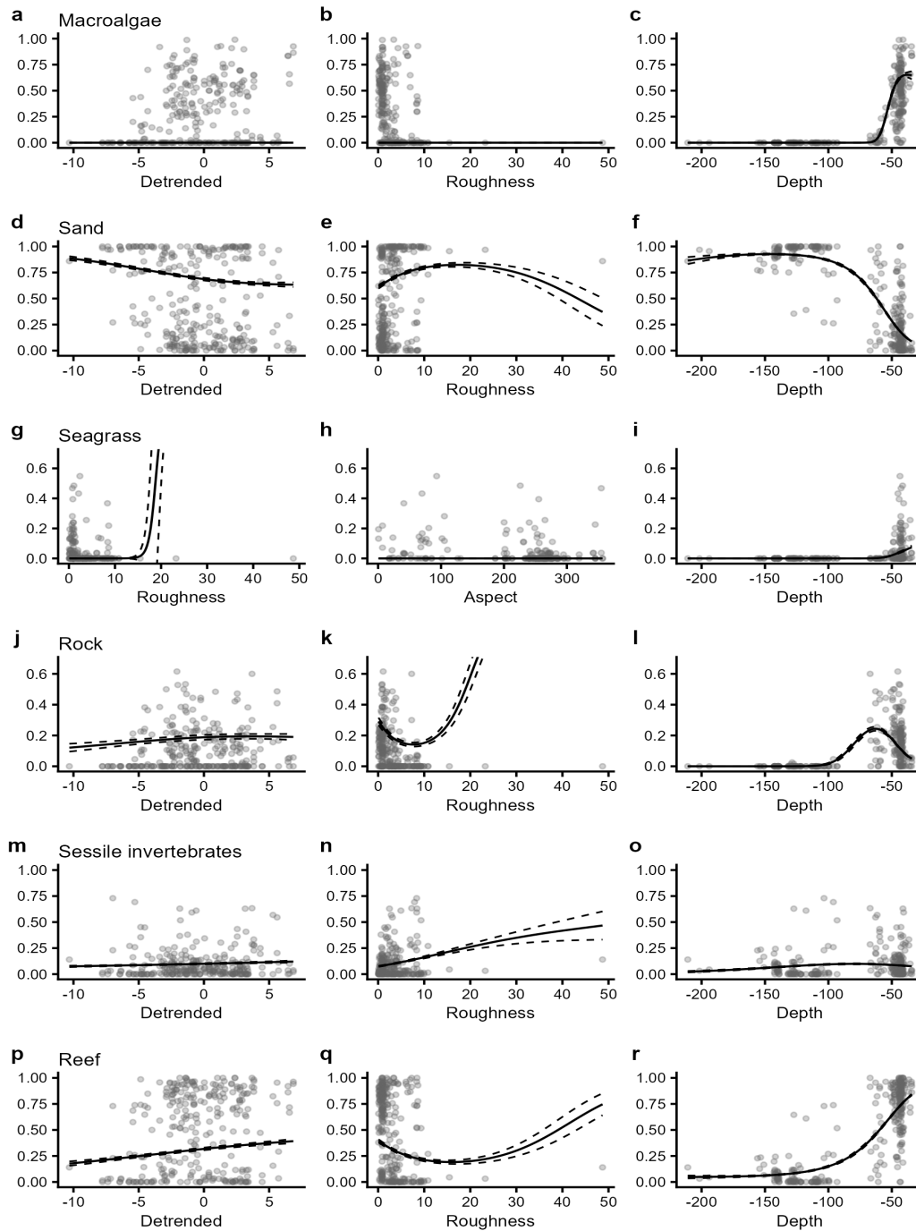
Figure C 1.2.1: Plots of the most parsimonious model found to predict the probability of occurrence of key habitat types in 2020. Individual panes display the predicted relationships between model covariates and the probability of occurrence of each habitat class. Solid lines represent predicted Generalized Additive Model (GAM) fits with other variables held constant at their mean value and survey year held at 2020. Dashed lines represent upper and lower standard error bounds around the prediction, and points represent the observed data for that year.
